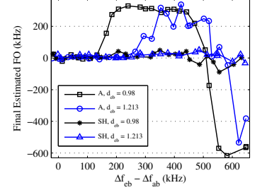
Fig. 11. USRP results: Final FO estimation error of the attack (A) and the sequence hopping scheme (SH).
