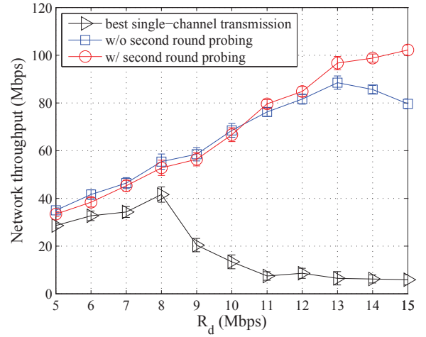
Fig. 14: Network throughput vs. R_d .
