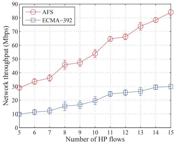
Fig. 13: Network throughput vs. L .
