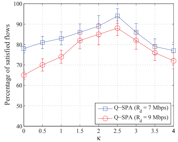
Fig. 10: Percentage of satisfied flows vs. \kappa .
