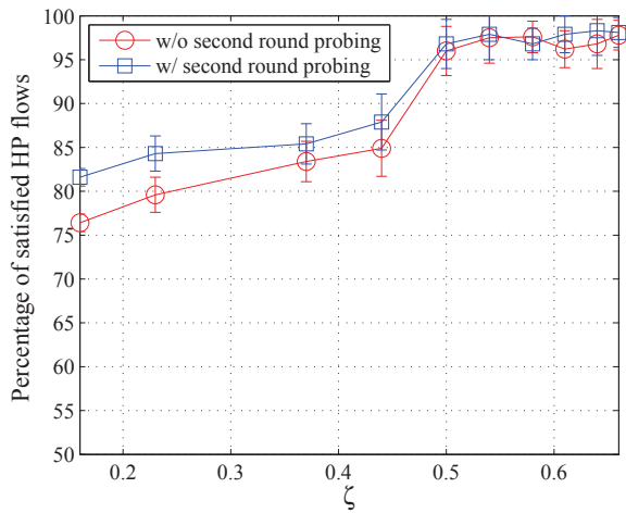
Fig. 15: Impact of second round probing.
