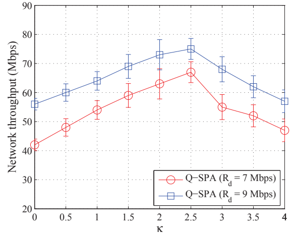
Fig. 9: Network throughput vs. \kappa .
