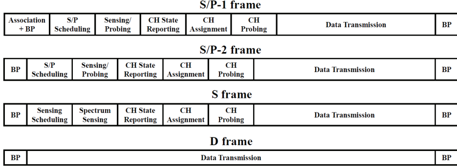
Fig. 2: Frame types used in AFS.
