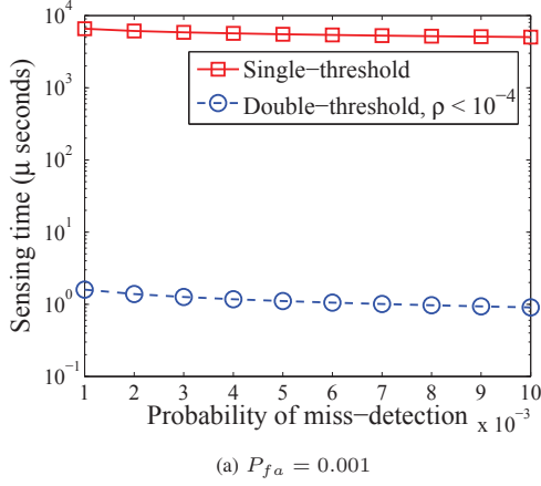
Fig. 4: Sensing time vs. (a) P_{md} and (b) P_{fa} ( P_{idle} = 0.5 , f_s = 6 MHz, and \gamma = -15 dB).
