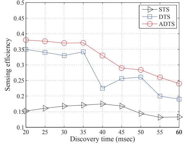
Fig. 7: Sensing efficiency.
