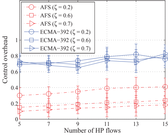
Fig. 11: Control overhead vs. L .
