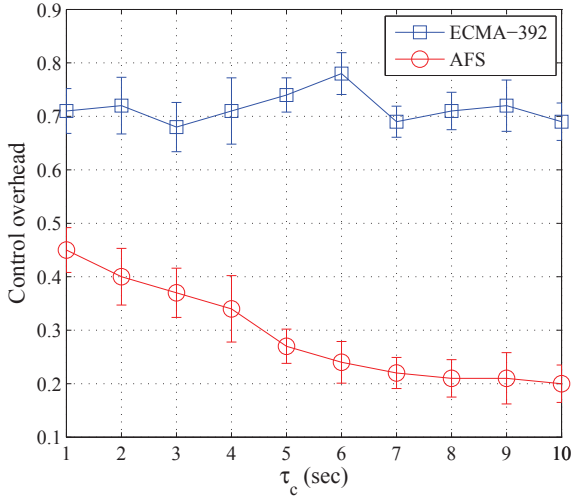
Fig. 12: Control overhead vs. \tau_c .
