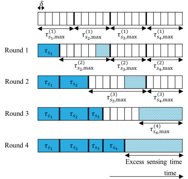
Fig. 5: An illustrative example for the adaptive sensing algorithm.
