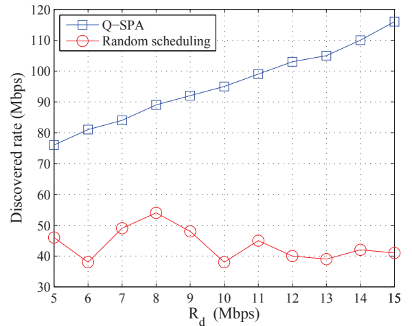
Fig. 8: Bandwidth discovered by QASPA.
