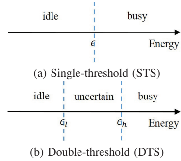
Fig. 3: Single- and double-threshold sensing approaches.
